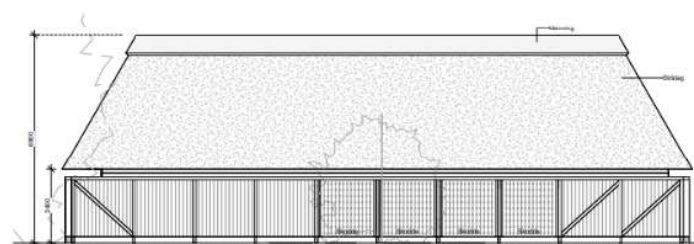
Facade N, laden 1 : 100
