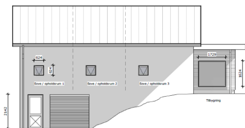
Facade Vest - 1 : 100
